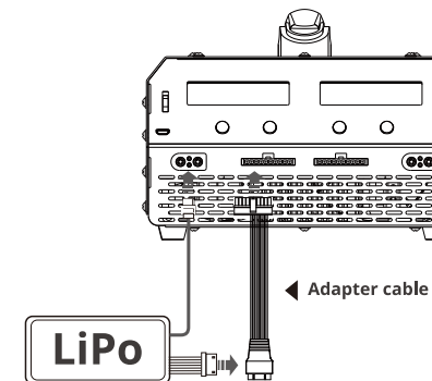
Direct Connecting Diagram
